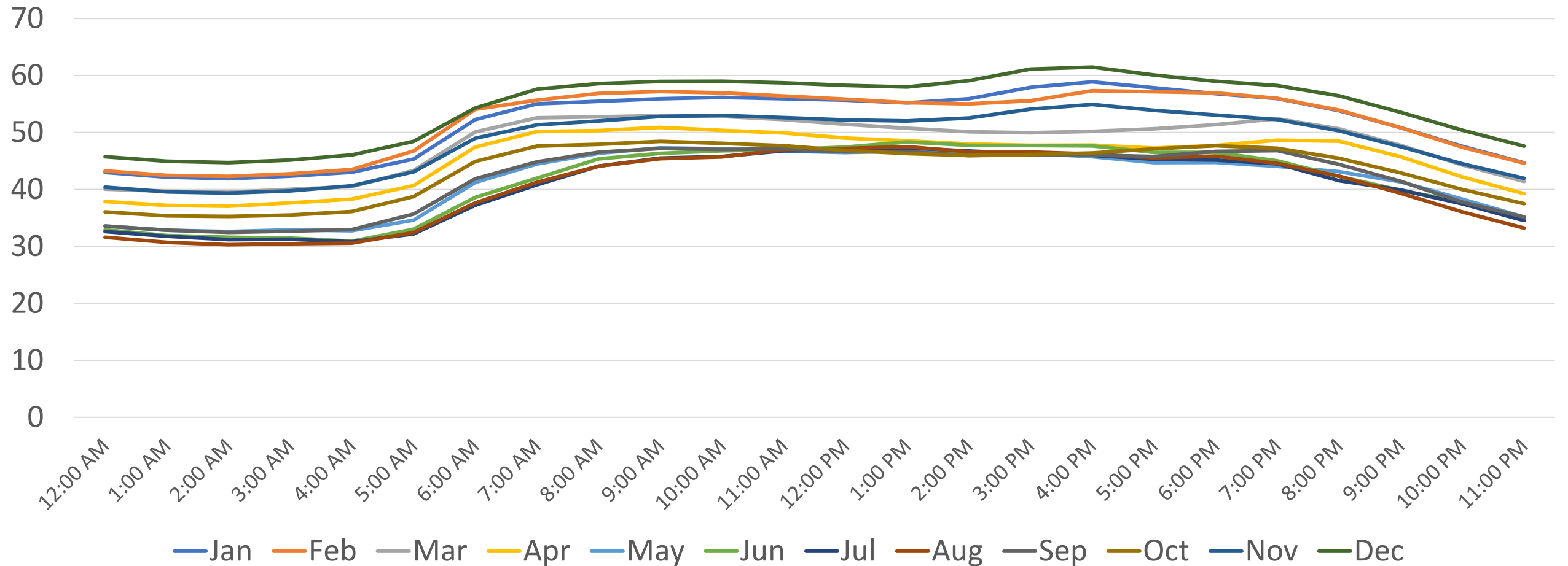
Average Hourly Loads by Month (MW)
